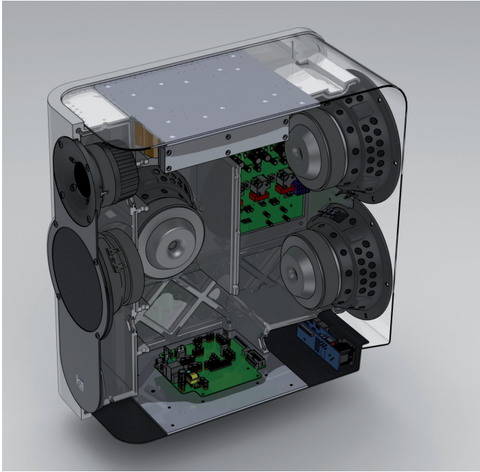
3D rendered interior view of the Kii Three Pro, right side shell and bass driver removed
