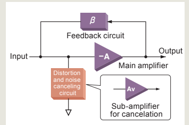
Block diagram of ANCC
